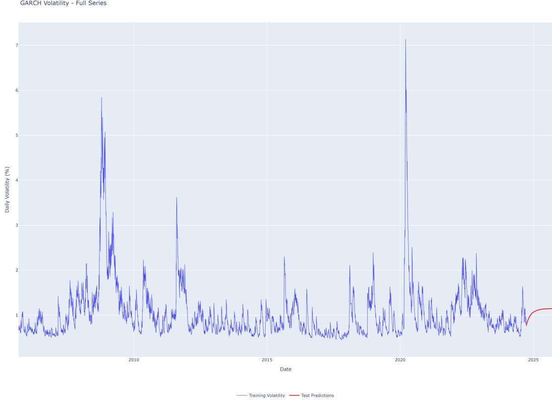
Figure 14: Trained Model Conditional Vol. and 1y Predicted Vol.
