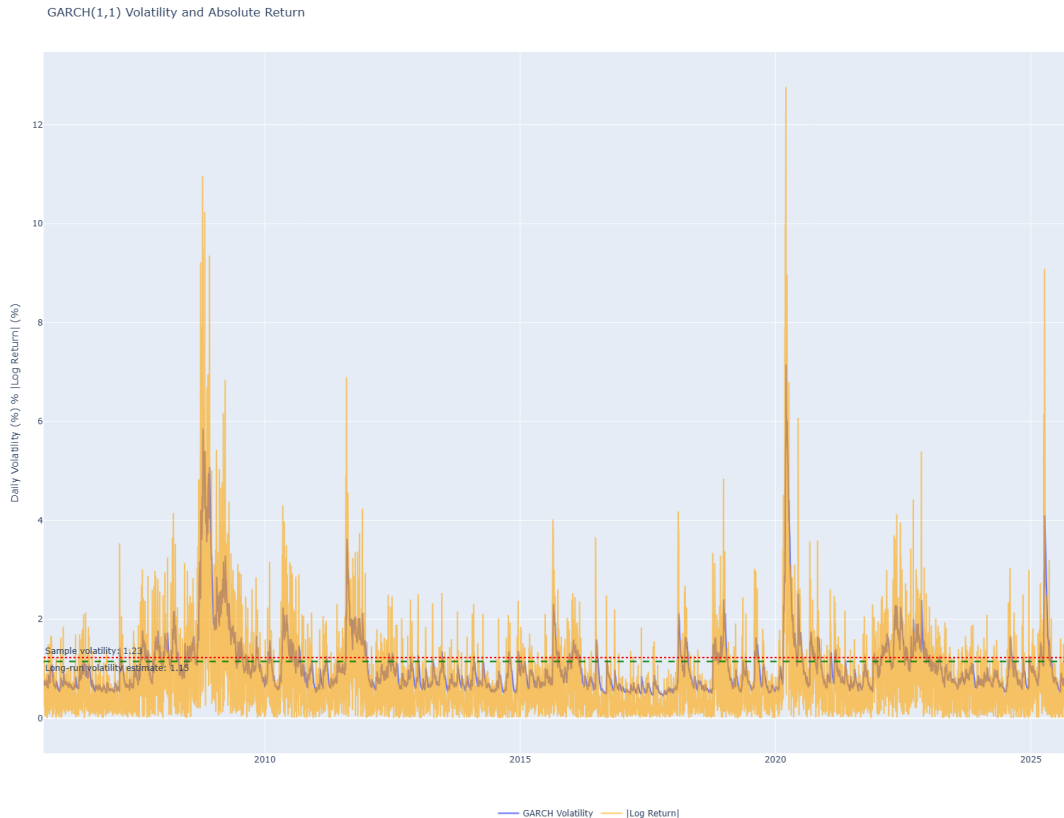
Figure 9: Volatility and Absolute Returns
