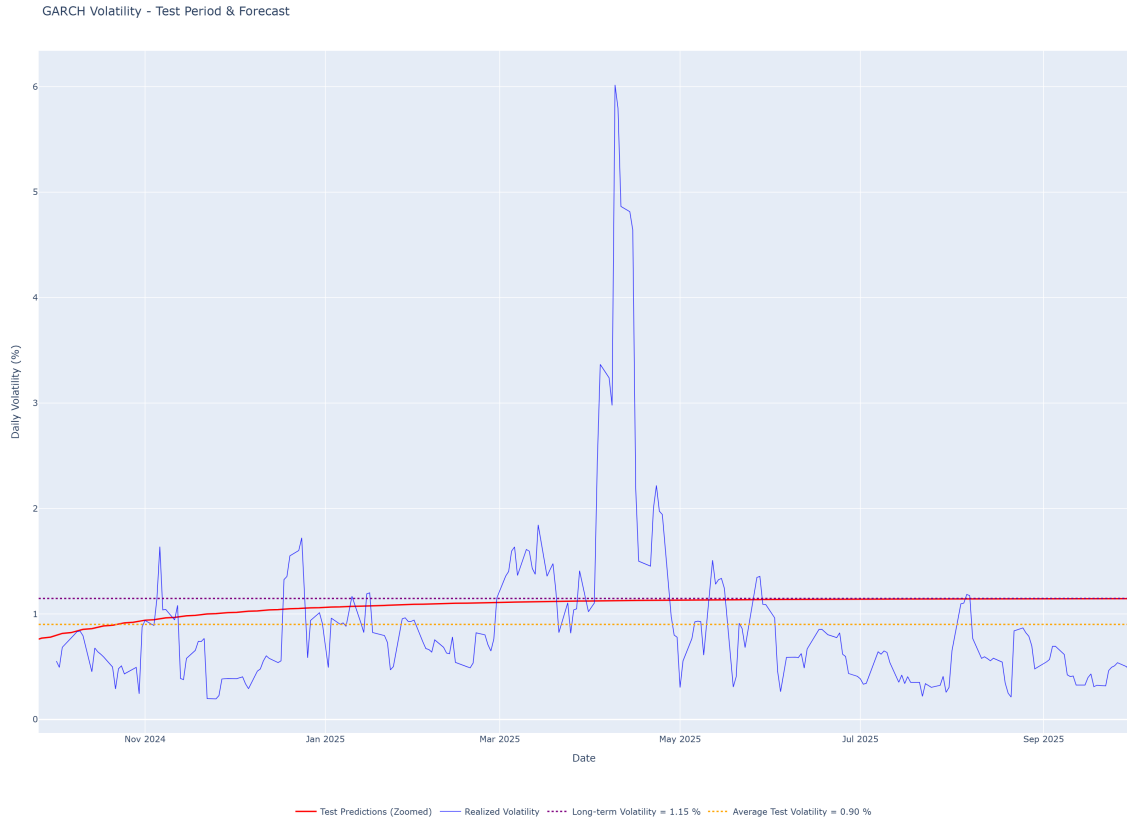
Figure 15: Test period: Prediction vs Realized volatility
