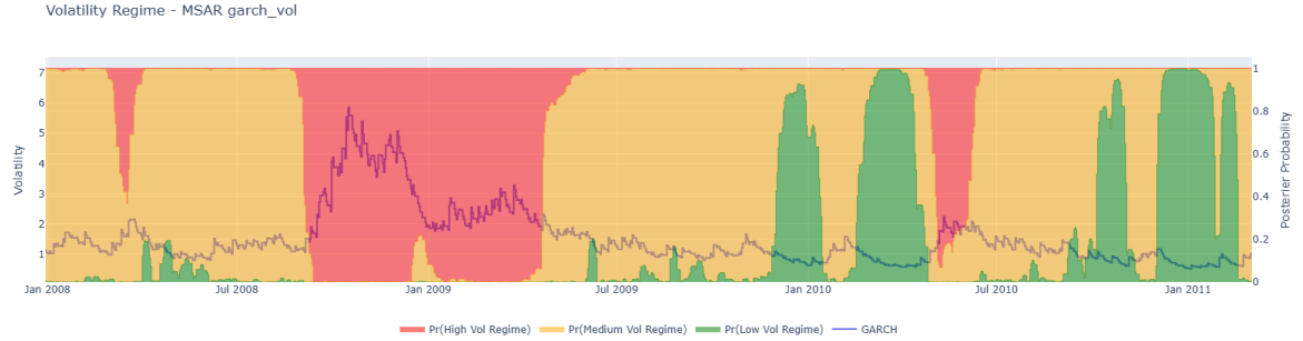
Figure 29: Zoomed MSAR Regime Classifier GARCH
