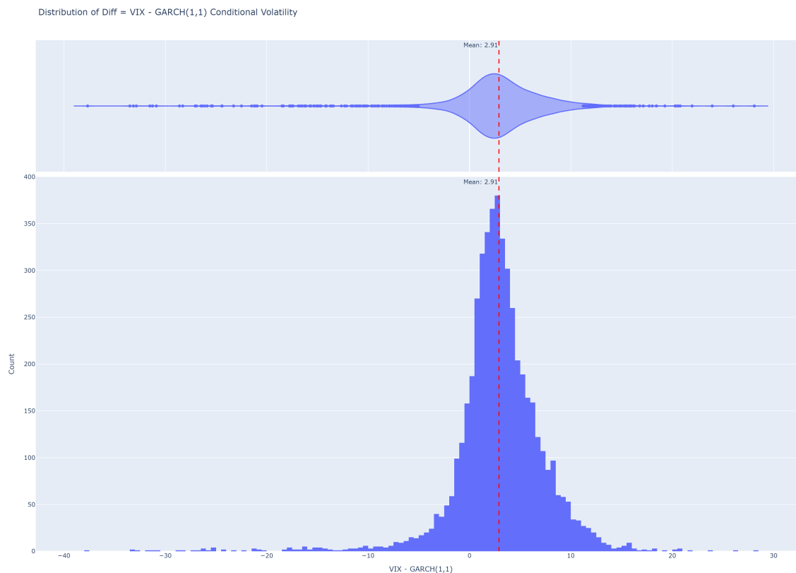
Figure 25: VIX - GARCH distribution
