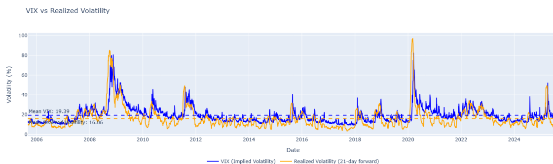
Figure 5: VIX vs Realized Volatility
