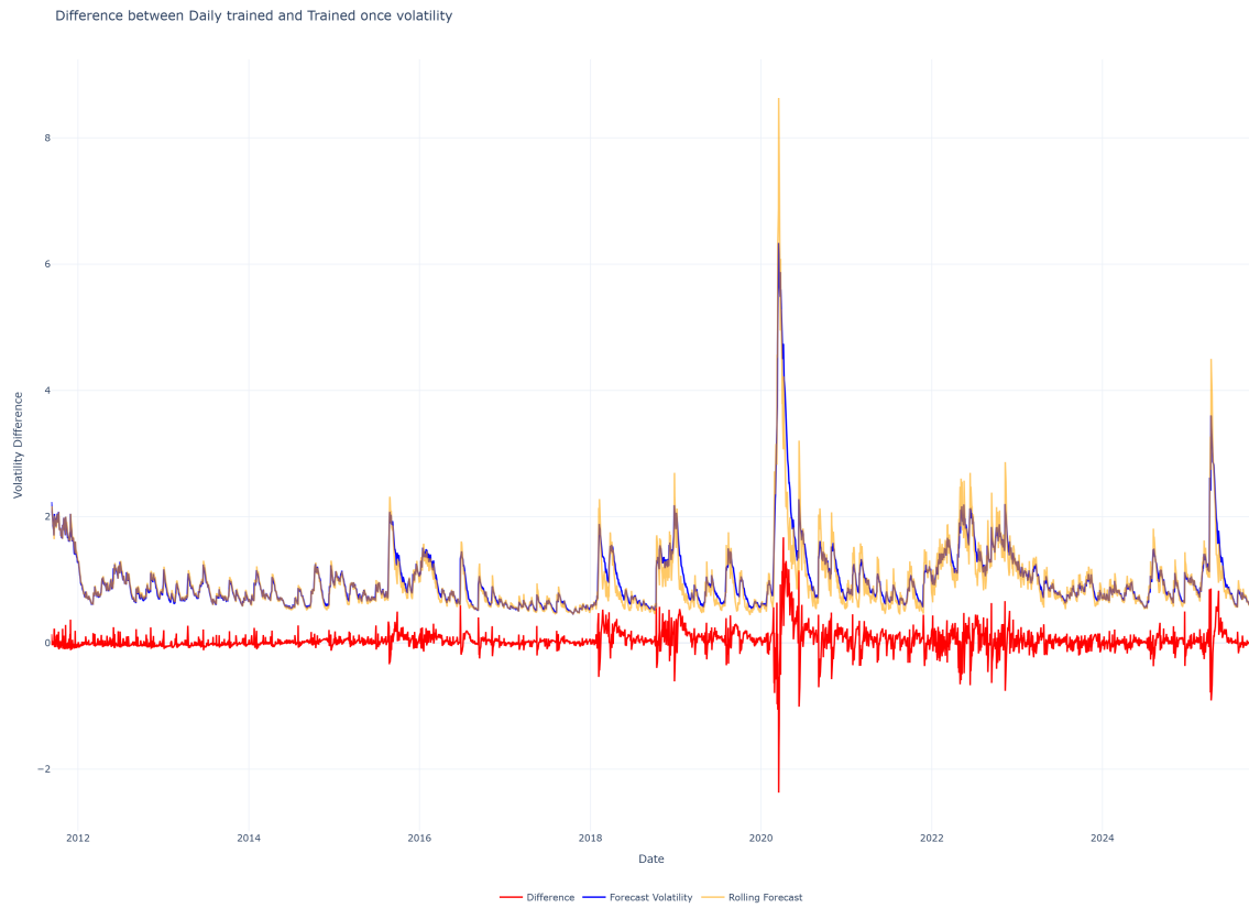
Figure 19: Daily trained vs Trained Once conditional volatilities
