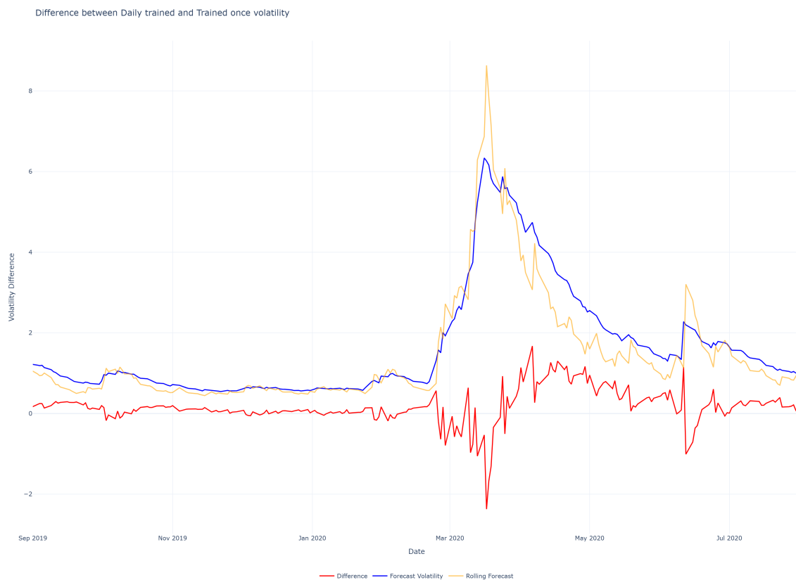
Figure 20: Zoomed Daily Trained model vs Trained Once model
