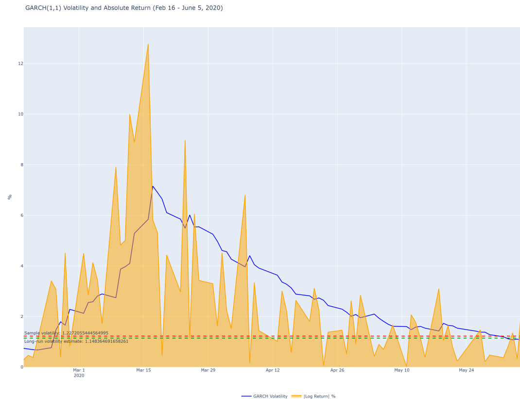
Figure 12: Persistence of volatility
