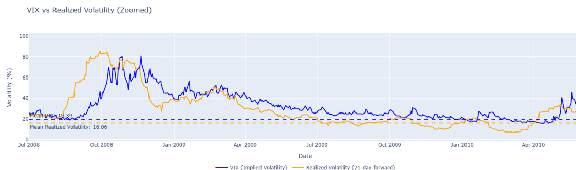
Figure 6: 2008 Crisis VIX vs Realized Volatility
