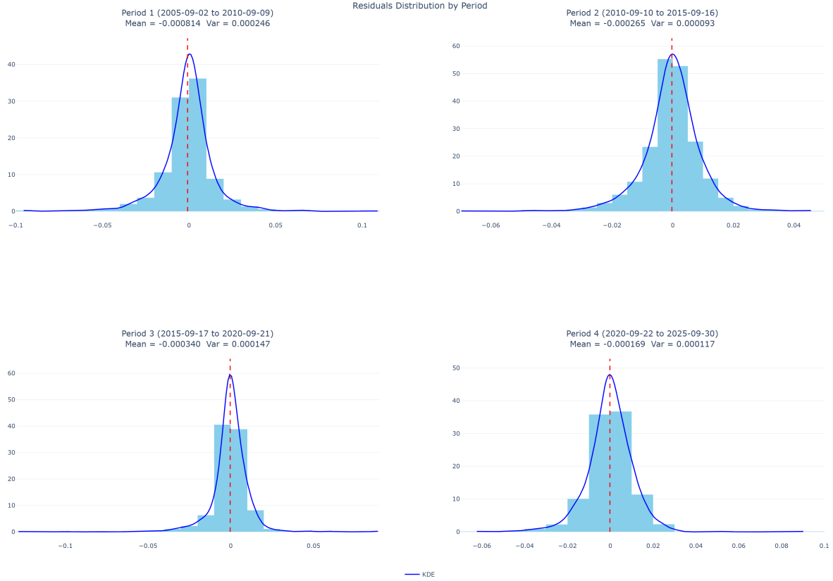
Figure 8: Distribution of shocks over the 4 periods
