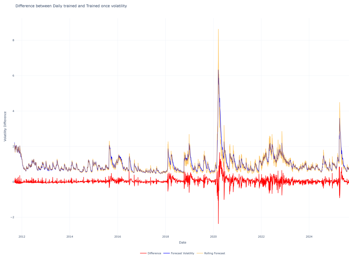
Figure 21: Difference between Daily Trained and Trained Once model volatility
