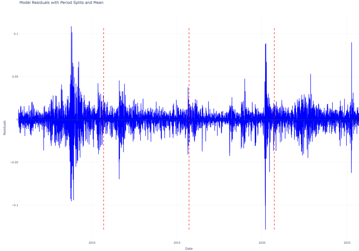
Figure 7: Residuals across time
