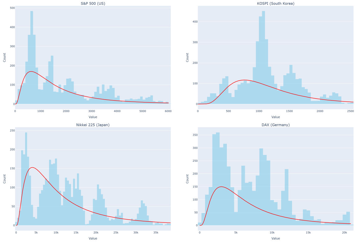
Figure 2: Log-Normal Prices Distribution
