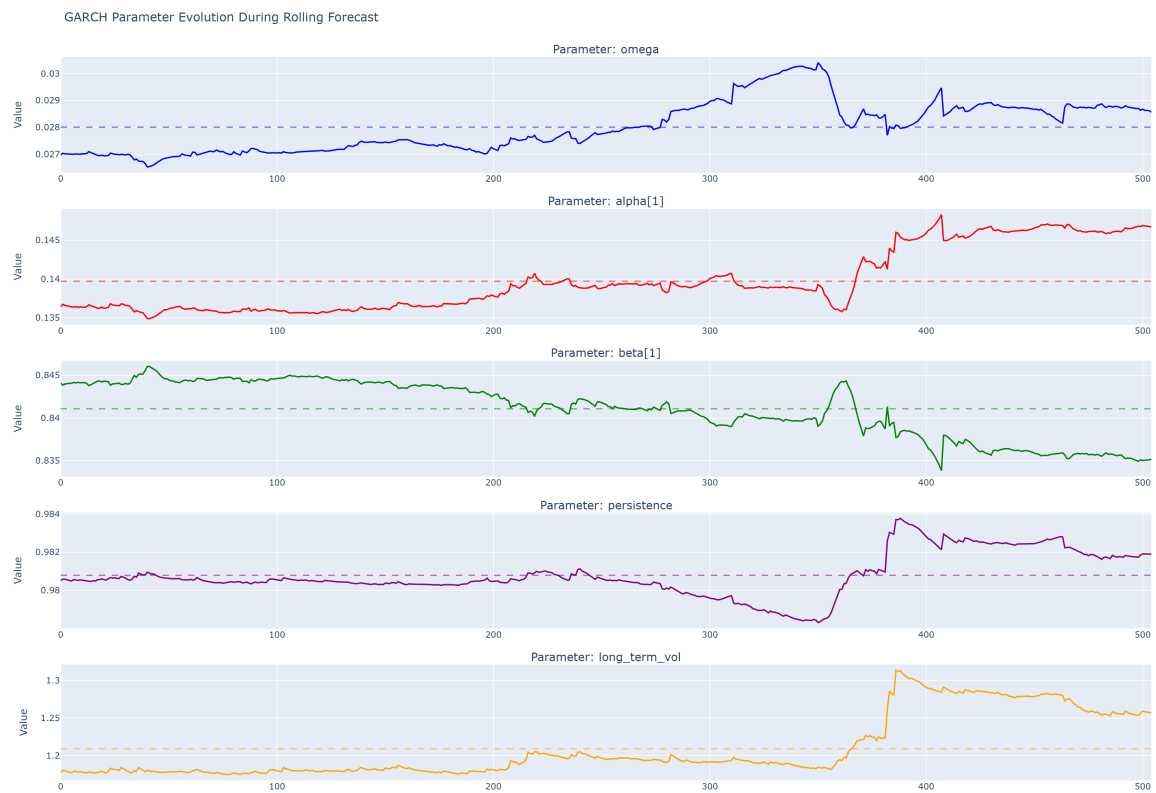
Figure 17: Parameter evolution over time
