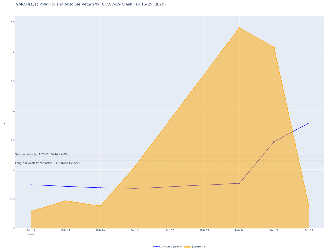
Figure 11: Lagged Conditional Volatility w.r.t abs. Returns
