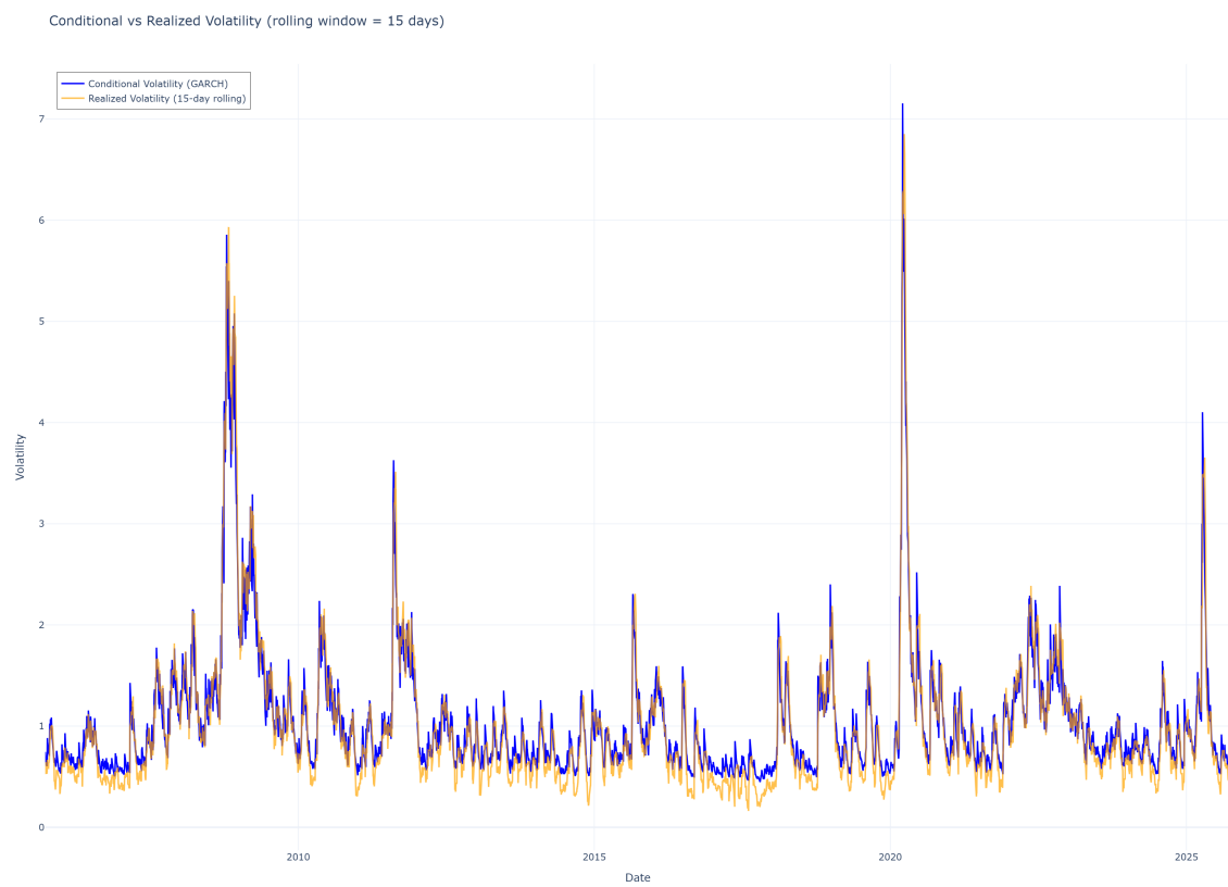
Figure 13: Conditional vs (Smoothed) Realized Volatility
