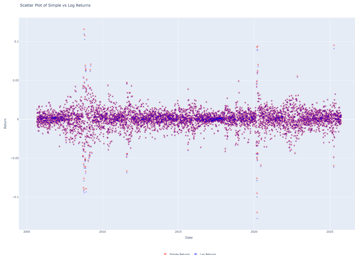
Figure 3: Simple vs Log Returns Scatter Plot
