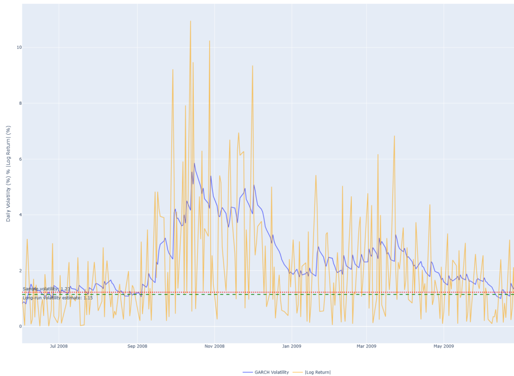
Figure 10: Absolute returns and Volatility (Zoomed in)
